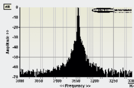
ABOVE: Wow and flutter re. 3150Hz tone at 5cm/sec (plotted ±150Hz, 5Hz per minor division). Wow is minimal but this deck was running imperceptibly fast
